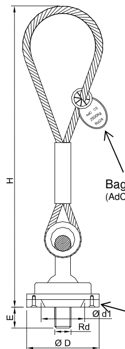
Bague amovible
